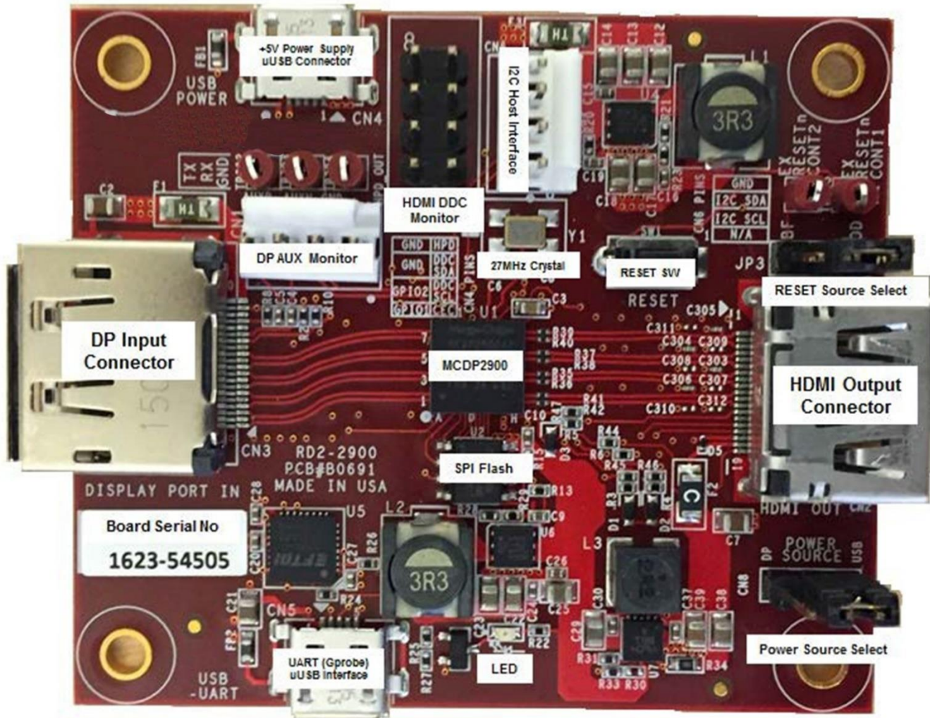
Figure 2. RD2-2900 Board Picture
