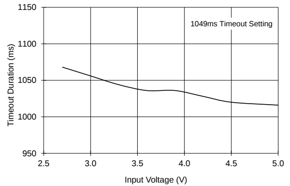
Timeout Duration vs. Input Voltage
