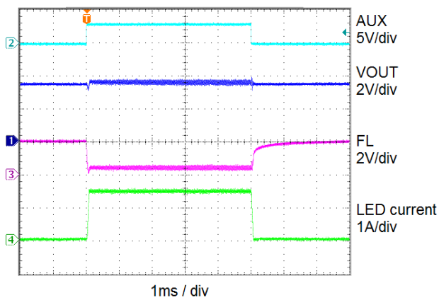
1.5A Flash with AUX (VIN = 3.6V)
