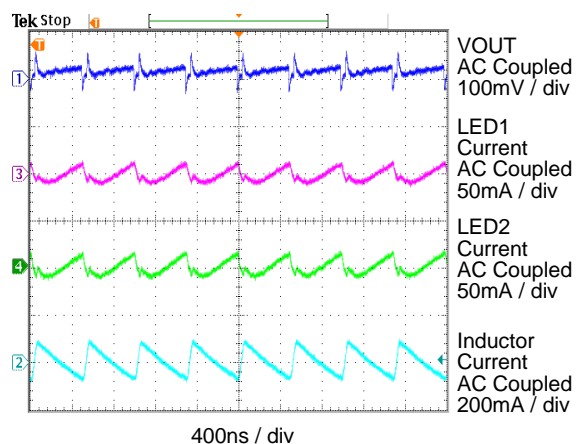
Switching Waveform at 2MHz
