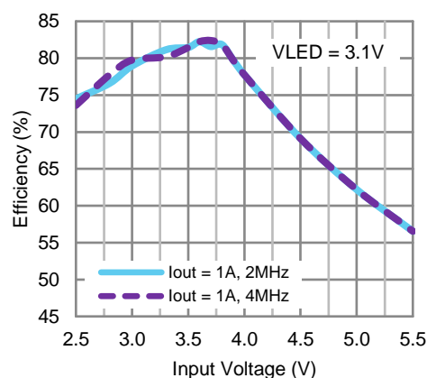
LED3 Efficiency vs. VIN (Torch Mode)
