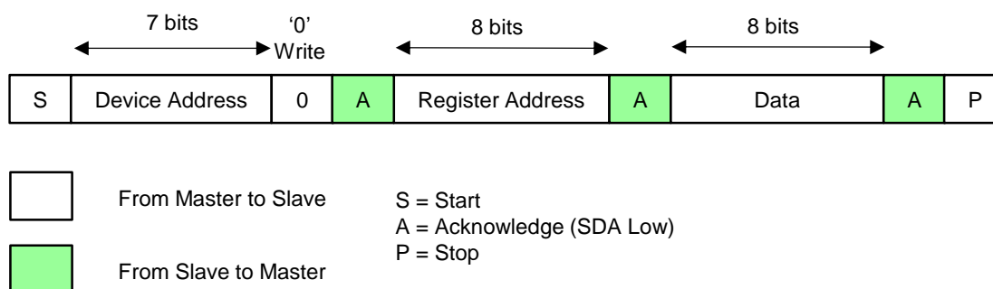
Figure 7. I²C Write Cycle
