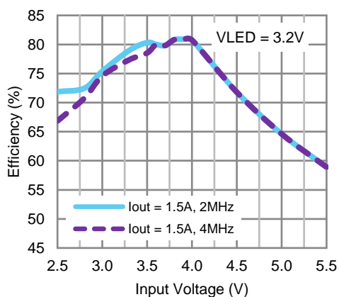
LED1 Efficiency vs. VIN (Flash Mode, 1.5A)
