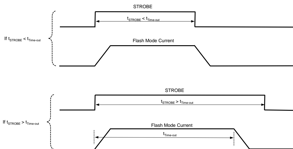
Figure 3. Flash Mode Current Controlled by STROBE (Level Triggered)
