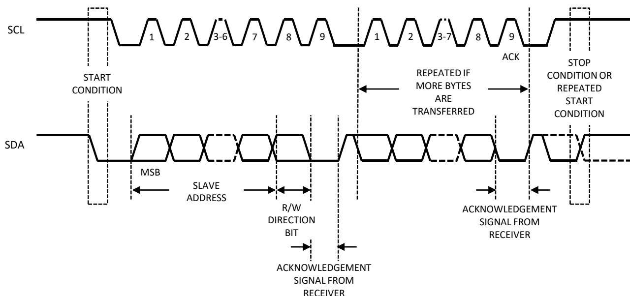
Figure 6. Data Transfer on I²C Serial Bus
