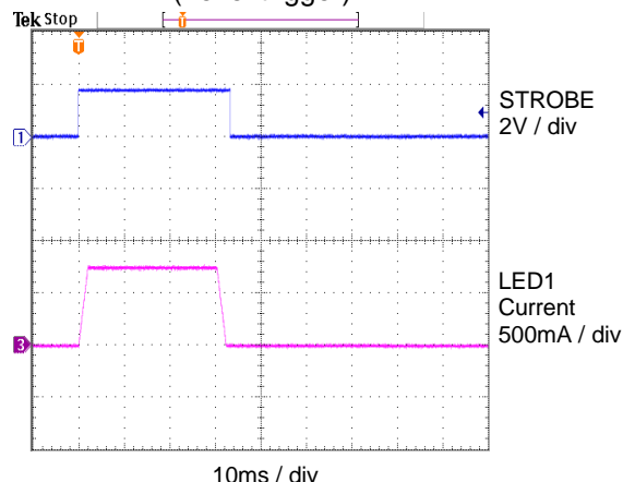
LED1 Torch on/off
