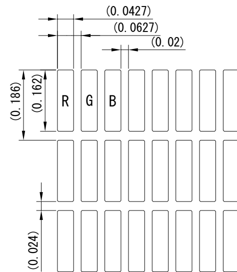
A部拡大図 (100:1) A-Portion Magnified Drawing (100:1)
