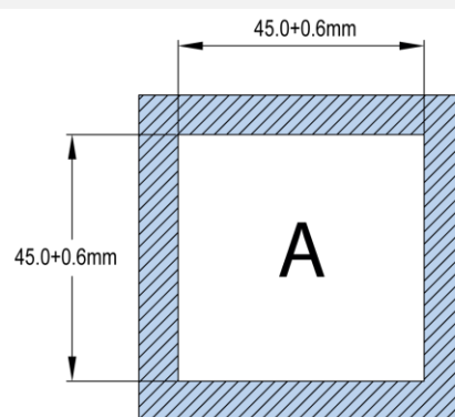
Panel Cut-Out
