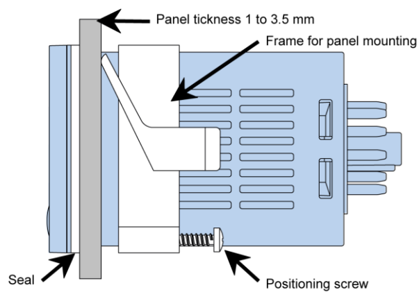
Mounting
