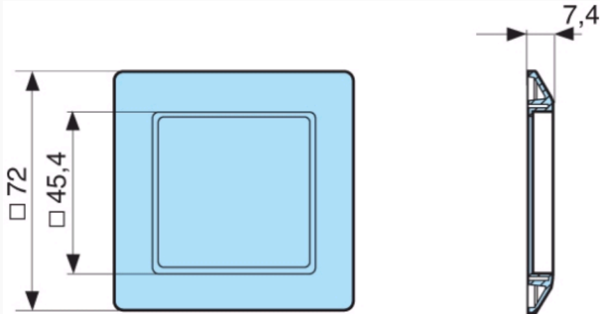
26546842 - Adaptor for 72 x 72 mm cut-out
