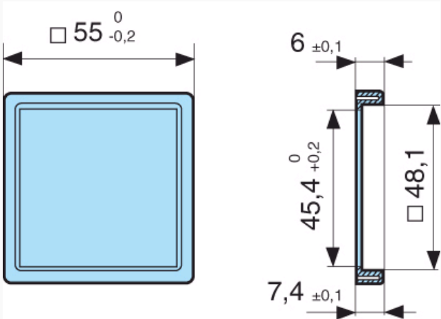
26546846 - Adaptor for 55 x 55 mm cut-out
