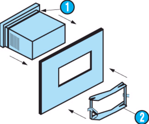
Fixing strip with clip-on yoke
