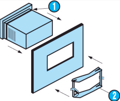
Fixing strip with clip-on yoke
