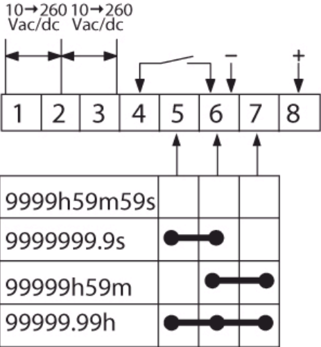
Start/Stop or reset input NPN - Transistor
