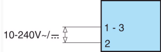
Start/Stop or reset input - Contact supplied with power
