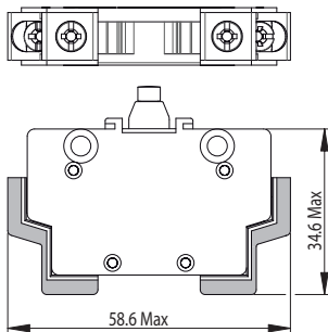
W5/IP20 screw with clamp and IP20 protection
