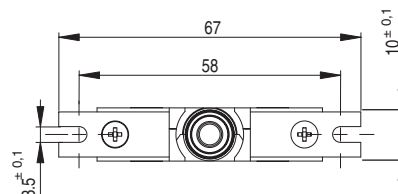
PE mounting plates with notches 79552460
