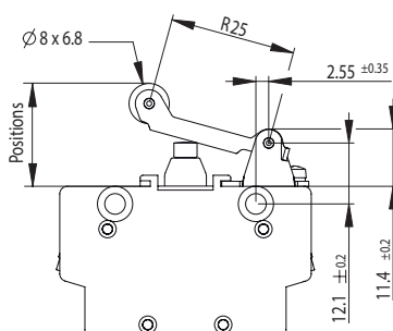
LG PE roller lever + plates with notches 79552458
