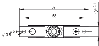
PT mounting plates with holes 79552459
