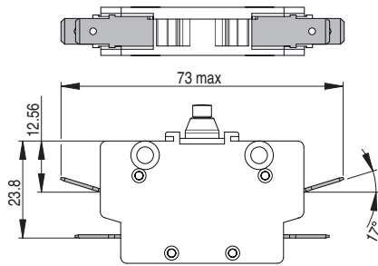
W3 quick-connect 6.3 x 0.8
