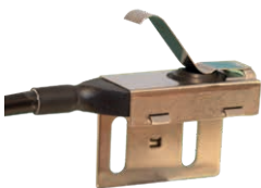
Angle mounting bracket and flexible lever for long overtravel.
