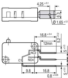
W3R5 quick-connect 6.3 x 0.8 for RAST 5 connector
