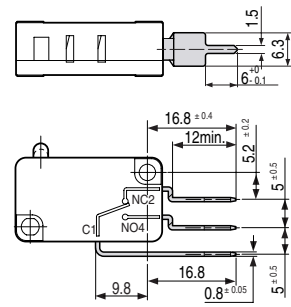
W3R2.5 for RAST 2.5 connector (SP9307)
