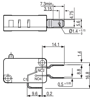
W6A5 quick-connect 4.8 x 0.5
