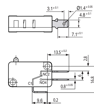
W6D8 quick-connect 4.8 x 0.8
