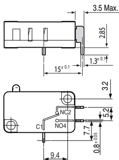
X3 for printed circuit board, front output
