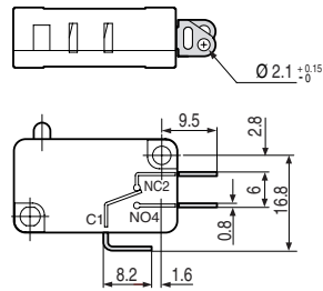
W6A5 quick-connect 4.8 x 0.5
