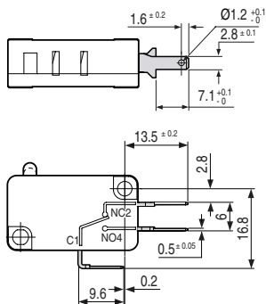
X3 for printed circuit board, front output
