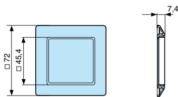
26546842 - Adaptor for 72 x 72 mm cut-out
