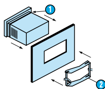
Fixing strip with clip-on yoke
