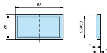
26546844 - Adaptor for cut-out
