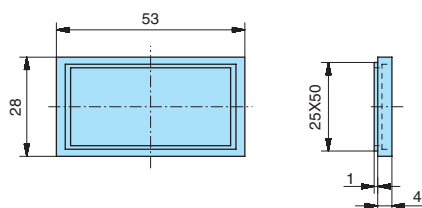
26546844 - Adaptor for 50 x 25 mm cut-out
