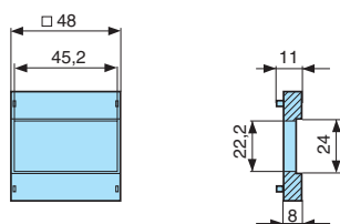
26546849 - Adaptor for 50 x 25 mm cut-out
