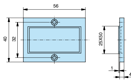
26546843 - Adaptor for cut-out
