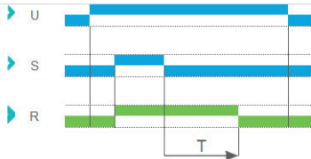
Function C - Off-Delay (Delay on break)
