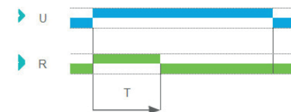
Function H - Interval
