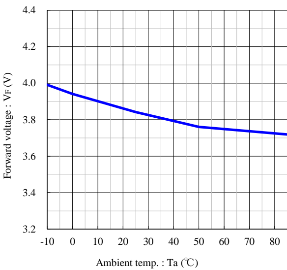
Ambient temp. vs. Forward voltage
