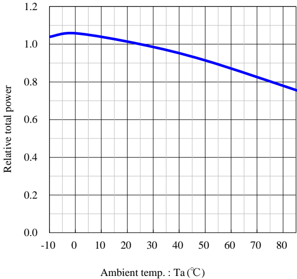
Ambient temp. vs. Relative total power
