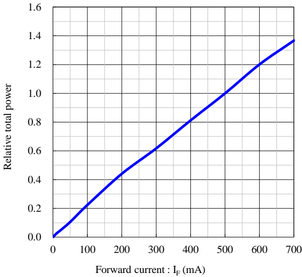
Forward current vs. Relative total power
