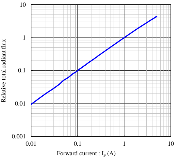
Forward current vs. Relative total radiant flux Condition : T_a = 25^{\circ}\text{C} , t_w = 100\mu\text{s}
