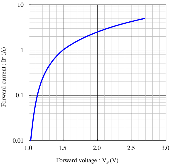
Forward voltage vs. Forward current Condition : T_a = 25^{\circ}\text{C} , t_w = 100\mu\text{s}
