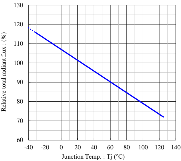
Junction temp. vs. Relative total radiant flux Condition : I_F = 1\text{A}
