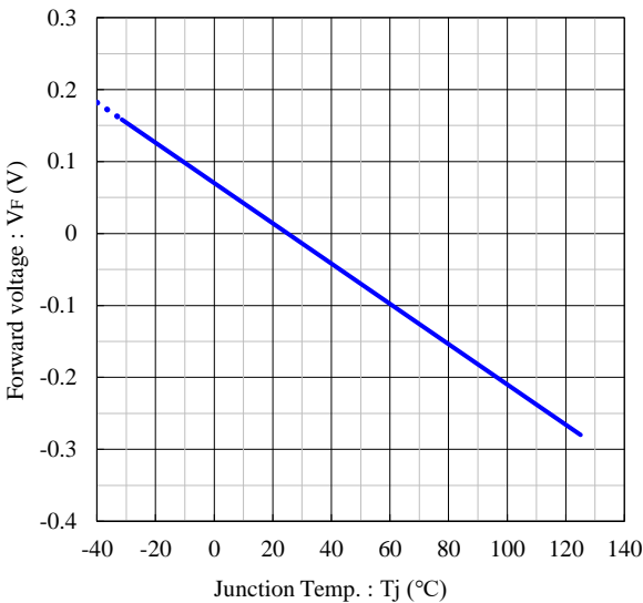
Junction temp. vs. Forward voltage Condition : I_F = 1\text{A}
