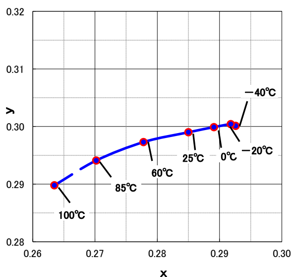
Ambient Temp. vs. Chromaticity coordinates
