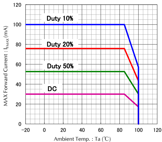
Ambient Temp. vs. Max. Forward Current Repetition Frequency : f \geq 10\text{Hz}
