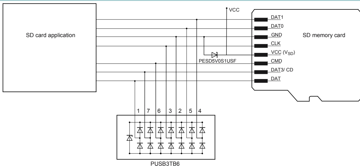
Fig. 11. Application diagram of SD card ESD protection using PUSB3TB6
