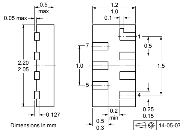
Fig. 12. Package outline XSON7 (SOT1358-1)
