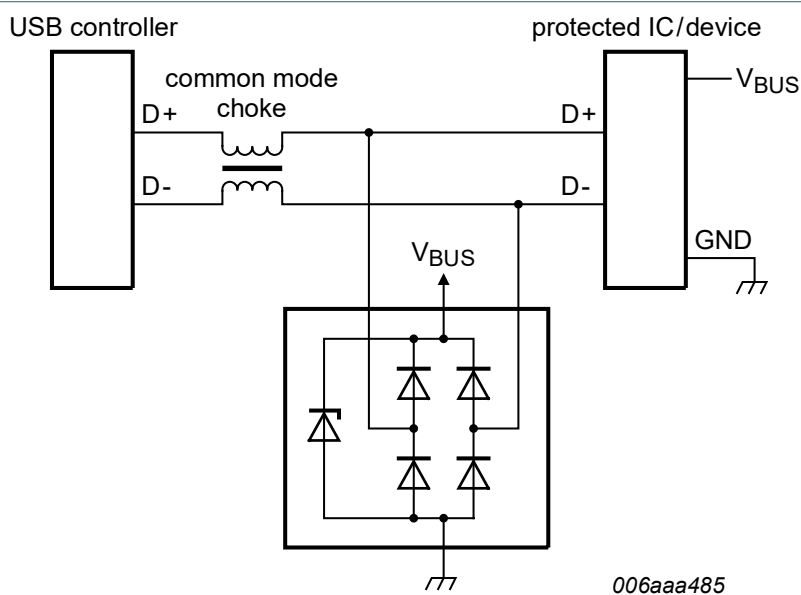
Fig. 4. Application diagram: USB 2.0
