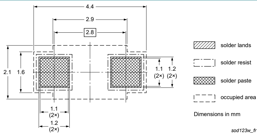
Fig. 15. Reflow soldering footprint for CFP3 (SOD123W)
