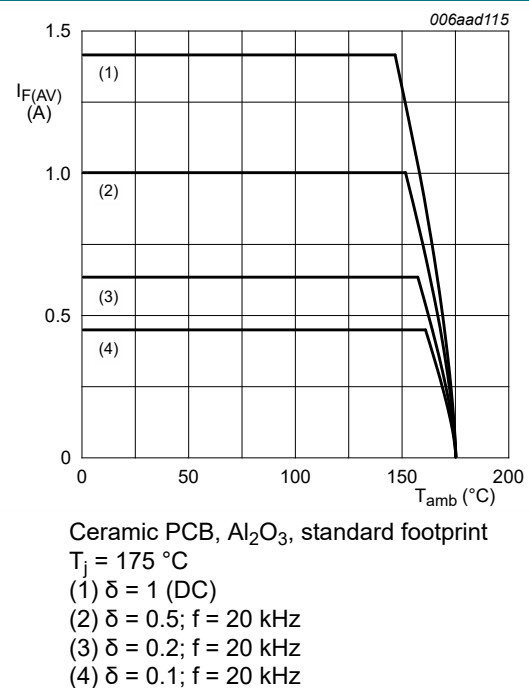
Fig. 13. Average forward current as a function of ambient temperature; typical values
