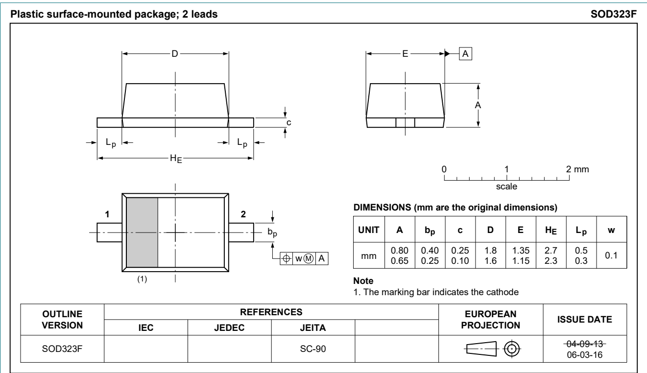
Fig. 5. Package outline SC-90 (SOD323F)
