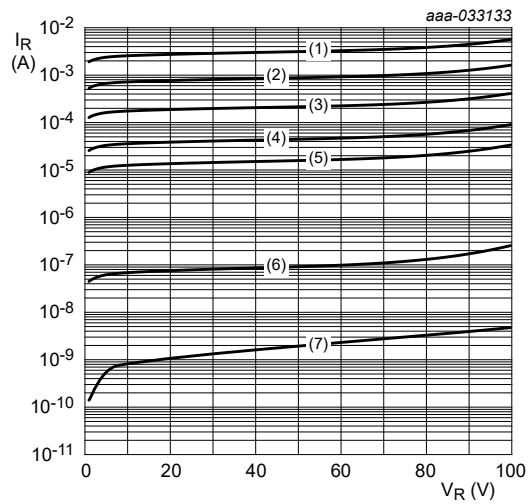
pulsed condition (1) T_j = 175^\circ\text{C} (2) T_j = 150^\circ\text{C} (3) T_j = 125^\circ\text{C} (4) T_j = 100^\circ\text{C} (5) T_j = 85^\circ\text{C} (6) T_j = 25^\circ\text{C} (7) T_j = -40^\circ\text{C}
