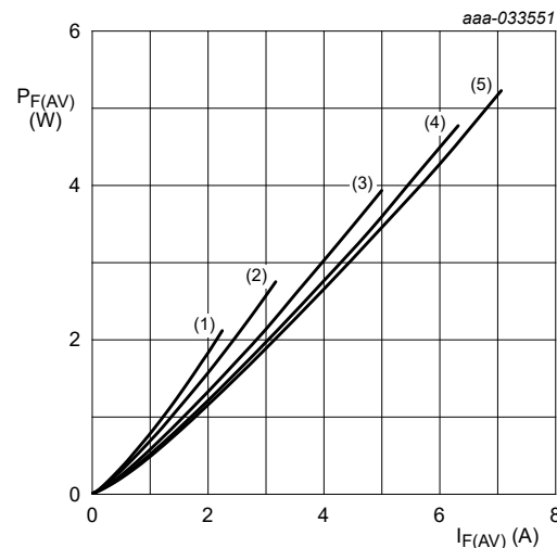
T_j = 100^\circ\text{C} (1) \delta = 0.1 (2) \delta = 0.2 (3) \delta = 0.5 (4) \delta = 0.8 (5) \delta = 1 ; DC
