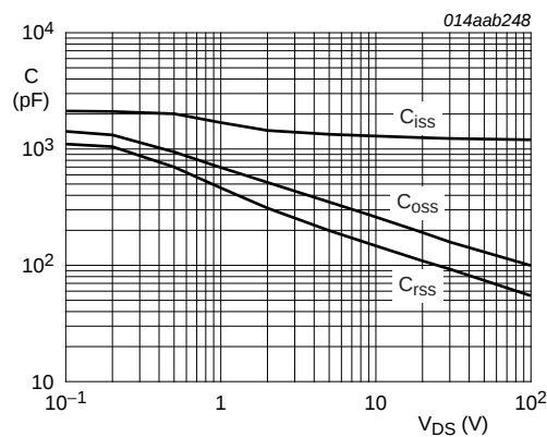
Fig 12. Input, output and reverse transfer capacitances as a function of drain-source voltage; typical values
