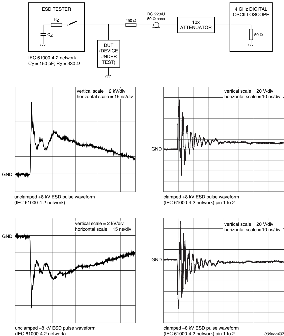
Fig 8. PESD9X7.0L: ESD clamping test setup and waveforms
