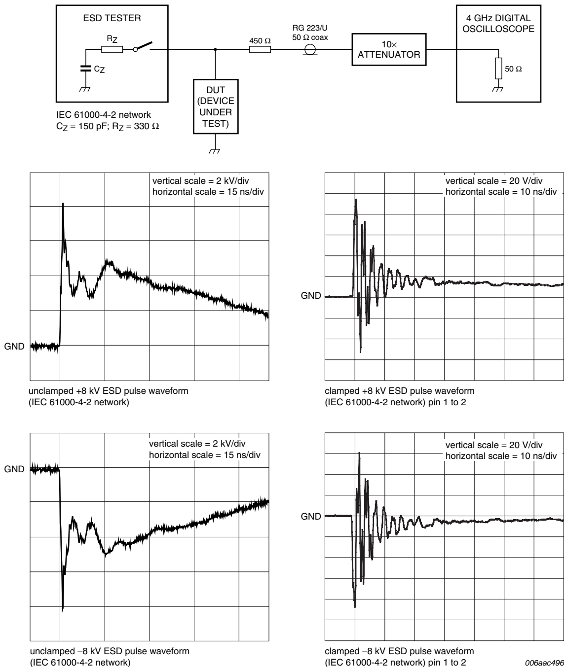
Fig 7. PESD9X5.0L: ESD clamping test setup and waveforms
