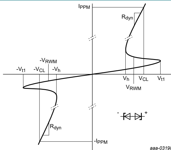
Fig. 3. V-I characteristics for a bidirectional ESD diode
