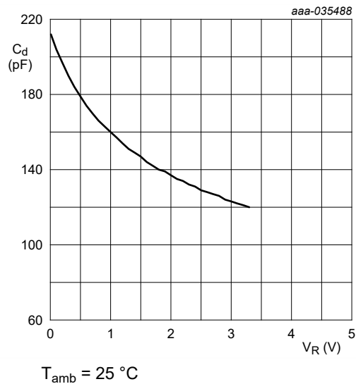
Fig. 5. Diode capacitance as a function or reverse voltage; typical values
