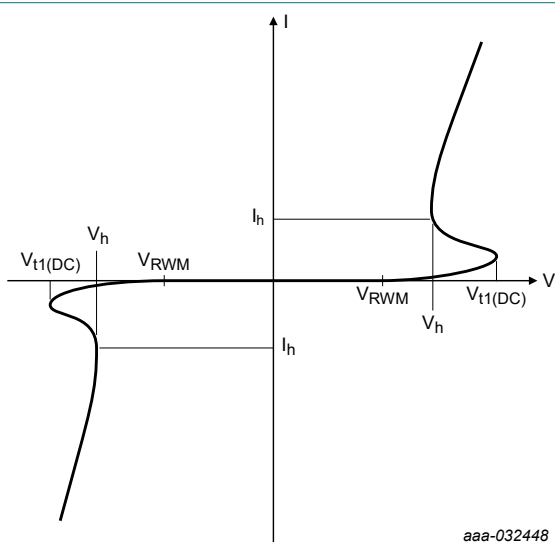
Fig. 3. Current forced I(V) characteristics for a bidirectional ESD protection device
