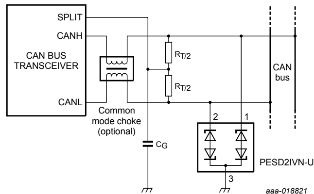
Fig. 10. Typical application: ESD protection of one automotive CAN bus line
