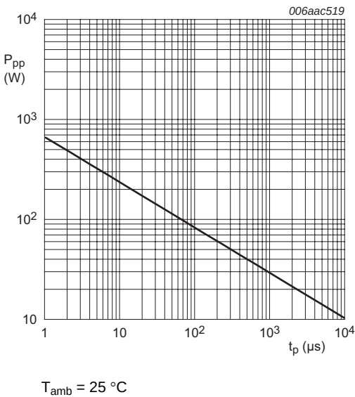
Fig 3. Peak pulse power dissipation as a function of pulse time; typical values
