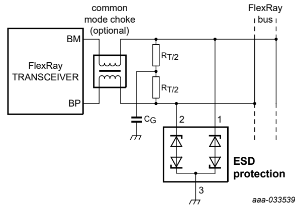
Fig. 7. Typical application: ESD protection of two automotive FlexRay data lines
