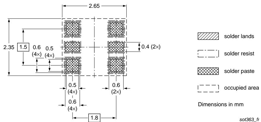
Fig 13. Reflow soldering footprint PUMH13 (SOT363)
