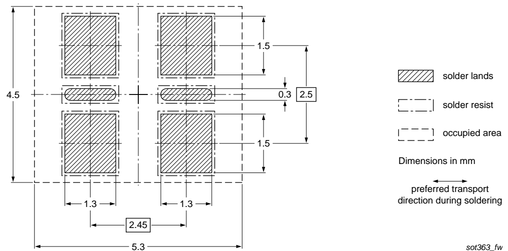
Fig 14. Wave soldering footprint PUMH13 (SOT363)
