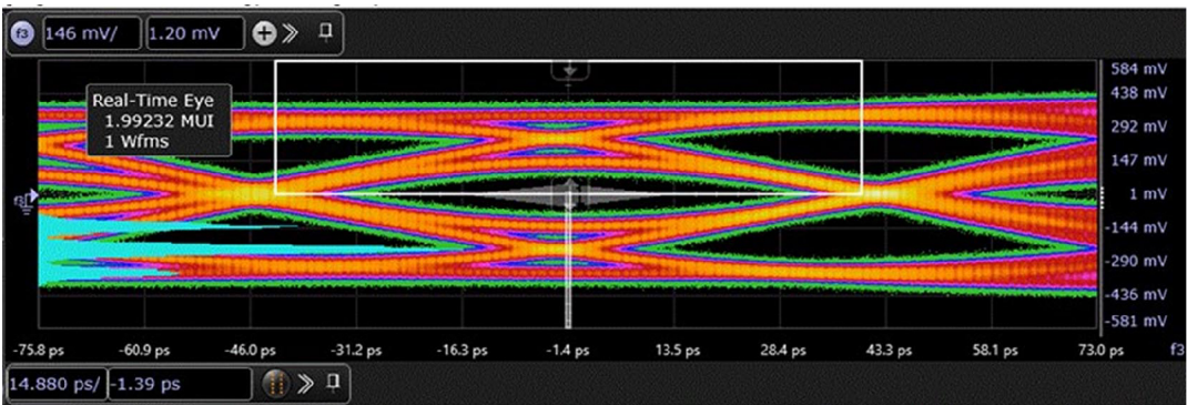
Fig. 7. HDMI 2.1 12G FRL eye diagram, PCB with device; typical values
