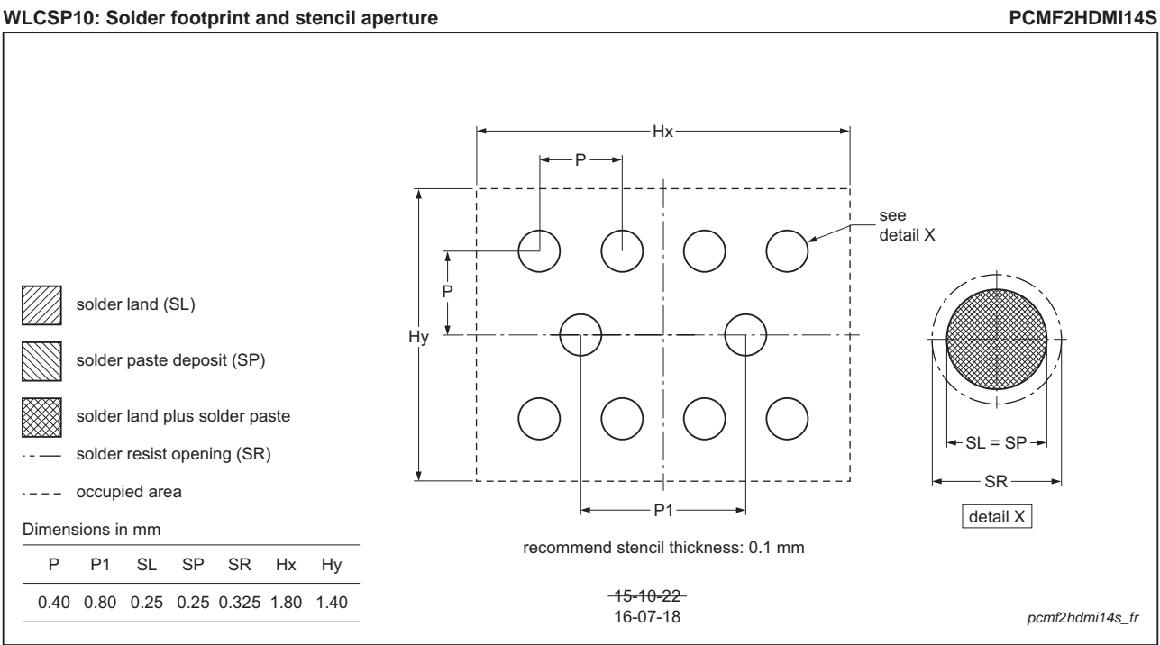
Fig 17. Soldering footprint WLCSP10 (PCMF2HDMI14S)
