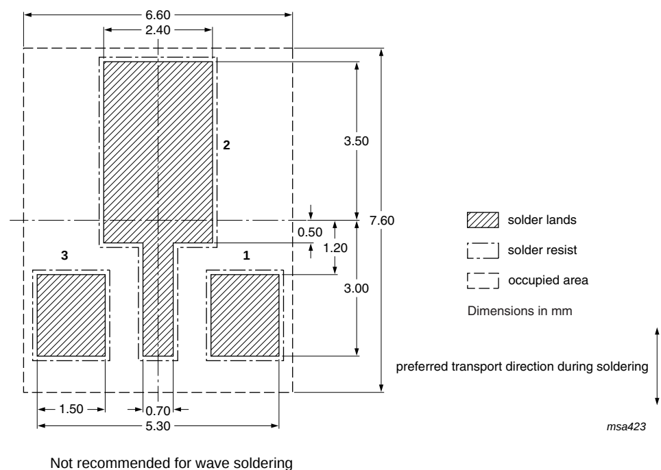
Fig 17. Wave soldering footprint SOT89 (SC-62)
