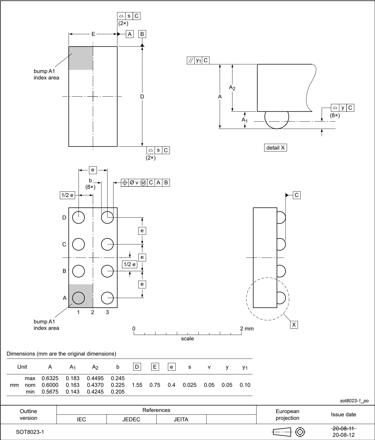
Fig. 14. Package outline SOT8023-1 (WLCSP8)
