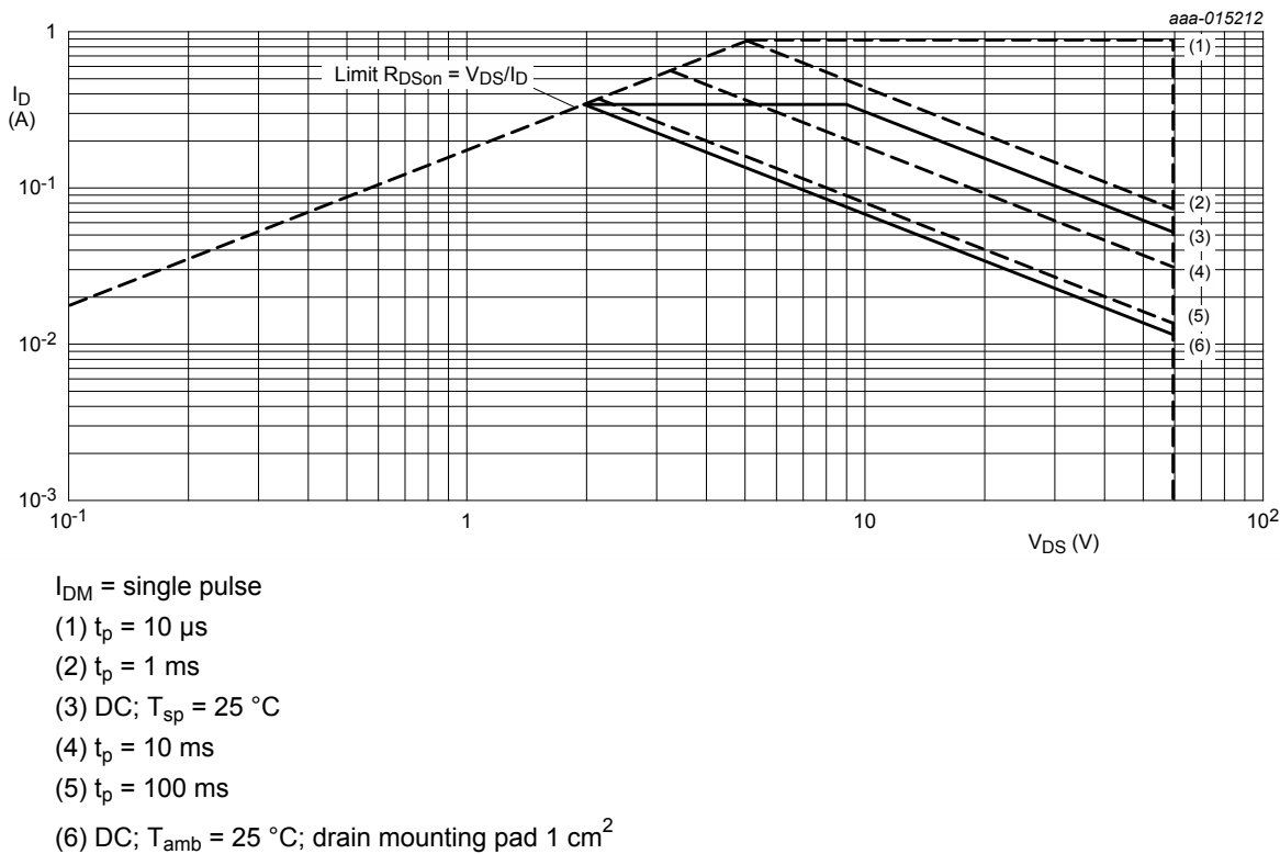
Fig. 4. Safe operating area; junction to ambient; continuous and peak drain currents as a function of drain-source voltage
