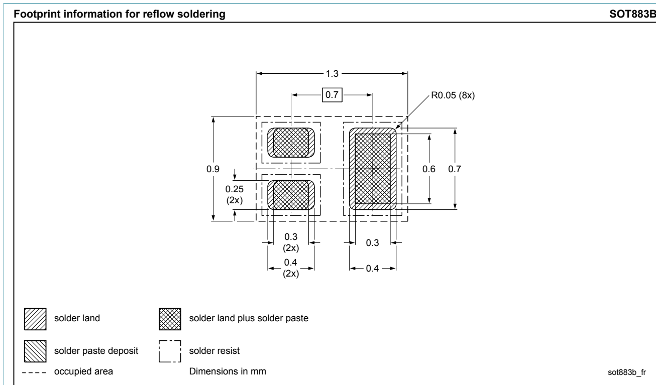
Fig. 20. Reflow soldering footprint for DFN1006B-3 (SOT883B)
