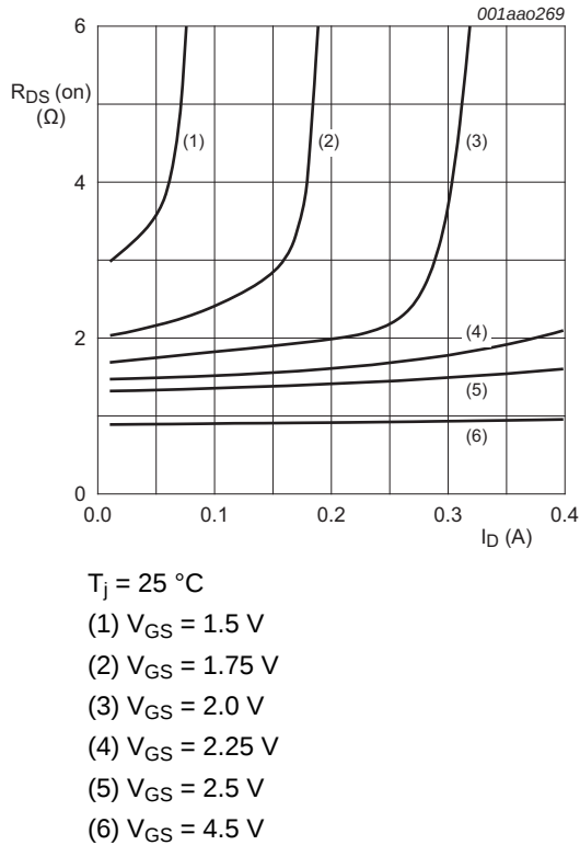
Fig 11. TR1: Drain-source on-state resistance as a function of drain current; typical values
