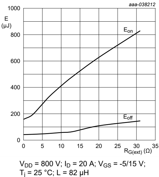
Fig. 15. Switching loss as a function of external gate resistance; typical values
