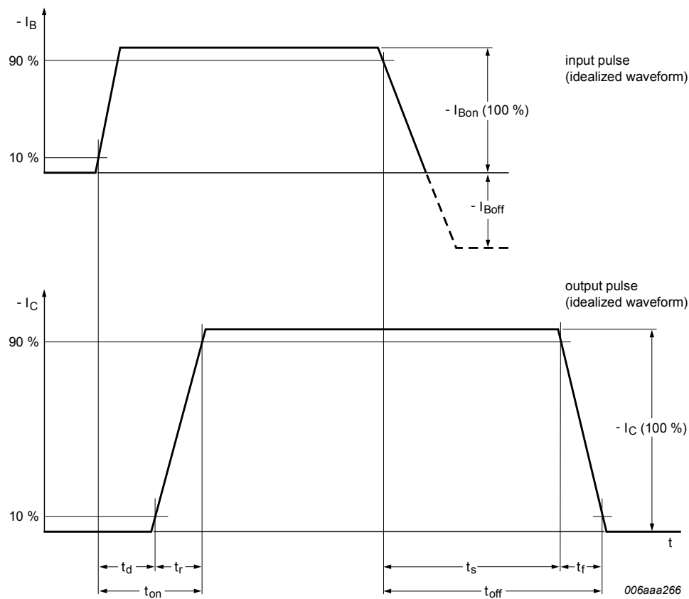
Fig. 16. TR2 (PNP): Transistor switching time definition
