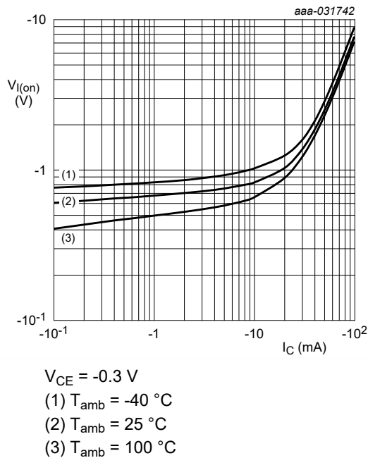
Fig. 11. NHUMD10, TR2 (PNP): On-state input voltage as a function of collector current; typical values
