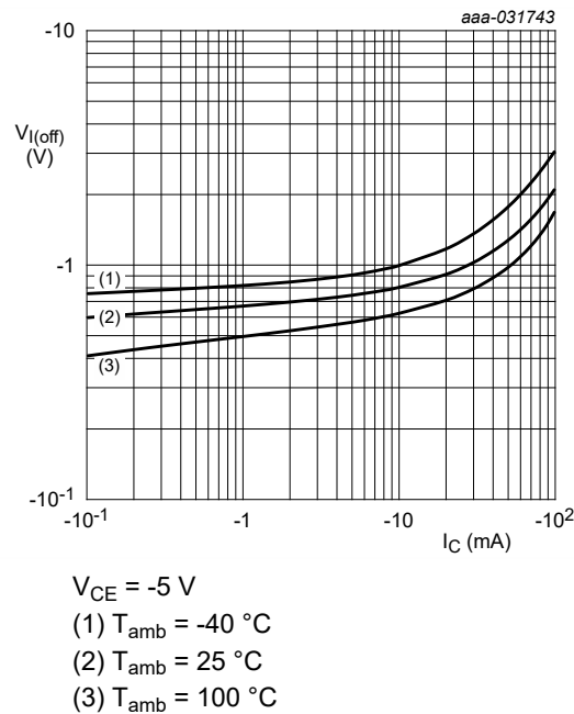
Fig. 12. NHUMD10, TR2 (PNP): Off-state input voltage as a function of collector current; typical values
