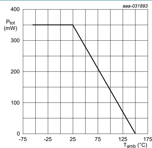
Fig. 1. Per device: Power derating curves for SOT363 (SC-88)
