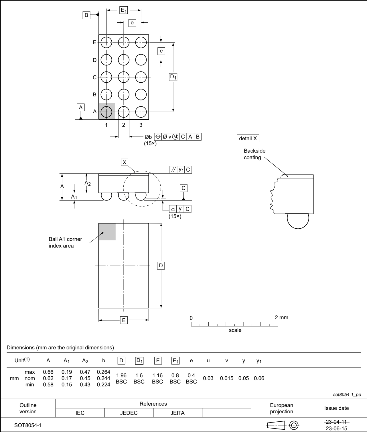
Fig. 41. Package outline SOT8054-1 (WLCSP15)
