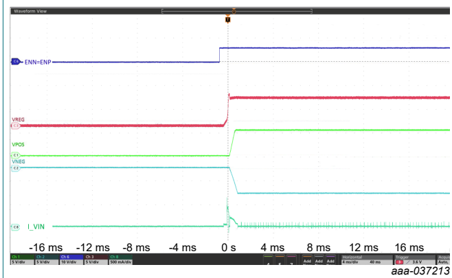
Fig. 32. Simultaneous power-up and inrush current
