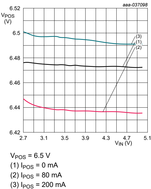
Fig. 18. V_{POS} versus V_{IN} line regulation
