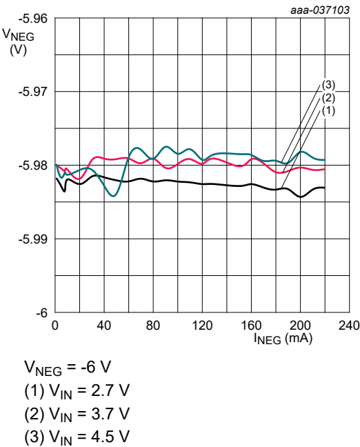
Fig. 23. V_{NEG} versus negative output current (load regulation)
