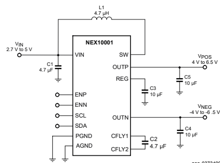
Fig. 1. Typical application
