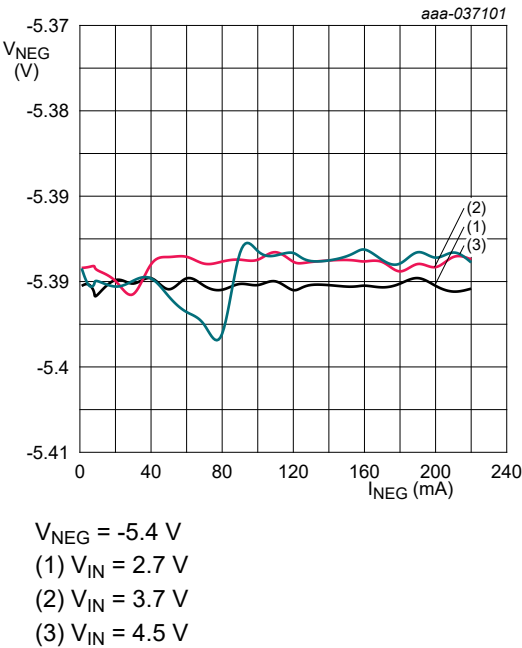
Fig. 21. V_{NEG} versus negative output current (load regulation)
