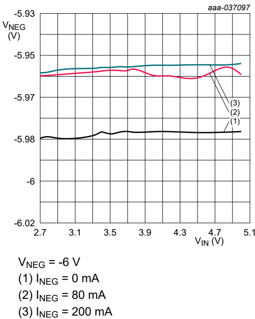
Fig. 17. V_{NEG} versus V_{IN} line regulation
