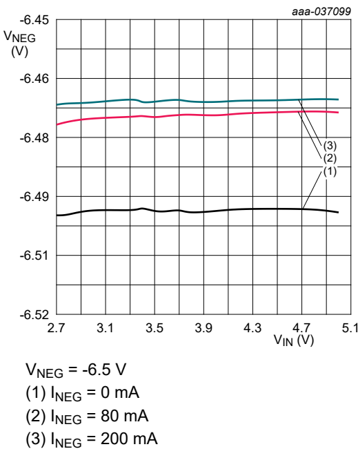
Fig. 19. V_{NEG} versus V_{IN} line regulation
