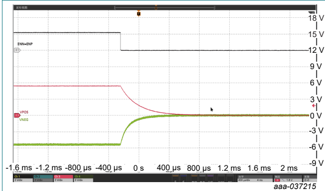
Fig. 34. Simultaneous shut-down
