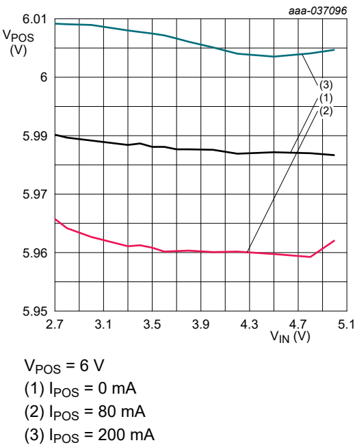
Fig. 16. V_{POS} versus V_{IN} line regulation
