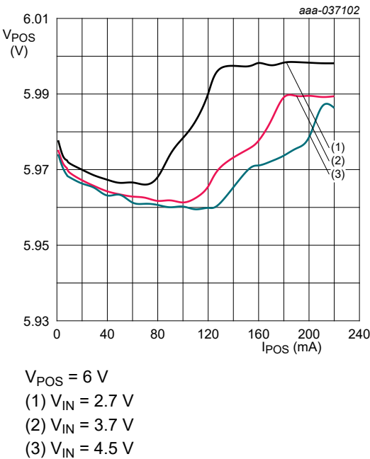
Fig. 22. V_{POS} versus positive output current (load regulation)
