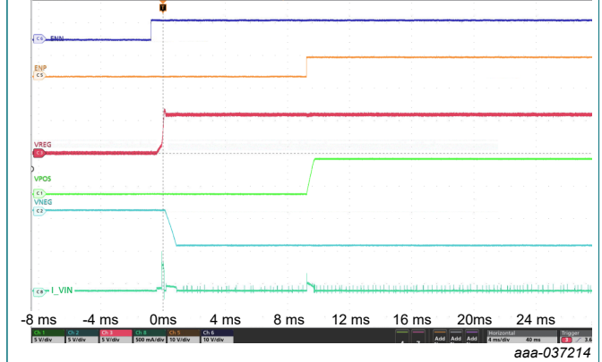
Fig. 33. Sequential power-up and inrush current
