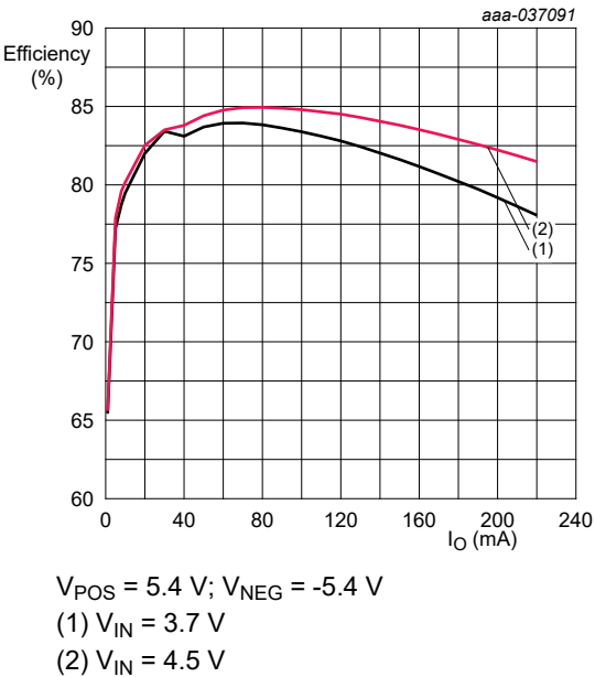
Fig. 11. Efficiency versus output current ( I_O )
