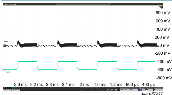
Fig. 34. Simultaneous shut-down
