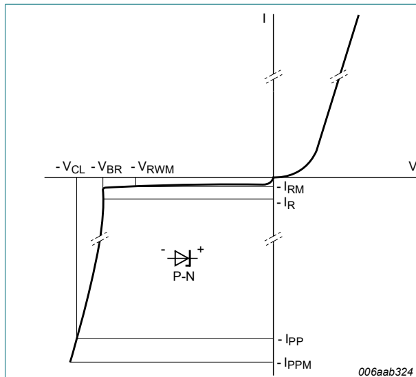
Fig. 4. V-I characteristics for a unidirectional TVS protection diode
