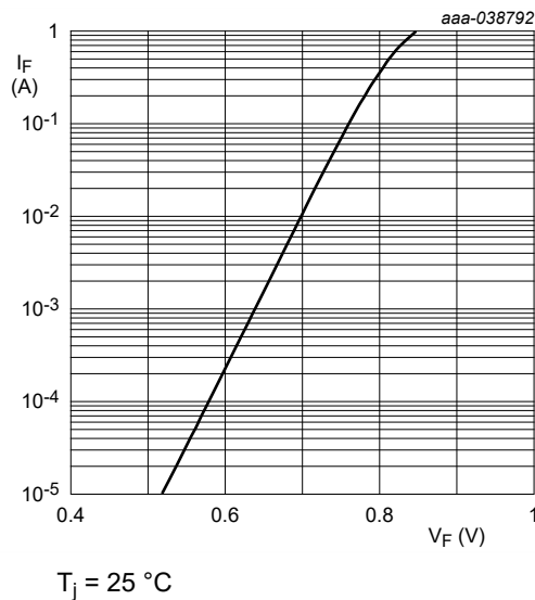
Fig. 3. Forward current as a function of forward voltage; typical values (HPZR-C3V3)
