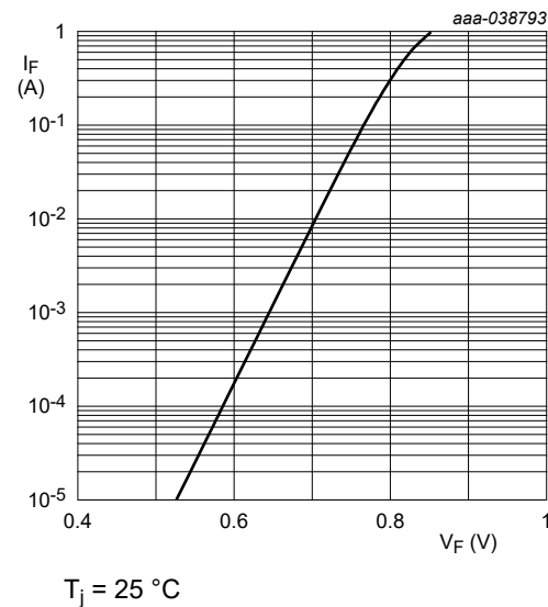
Fig. 4. Forward current as a function of forward voltage; typical values (HPZR-C5V1)
