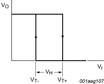
Fig. 6. Transfer characteristic
