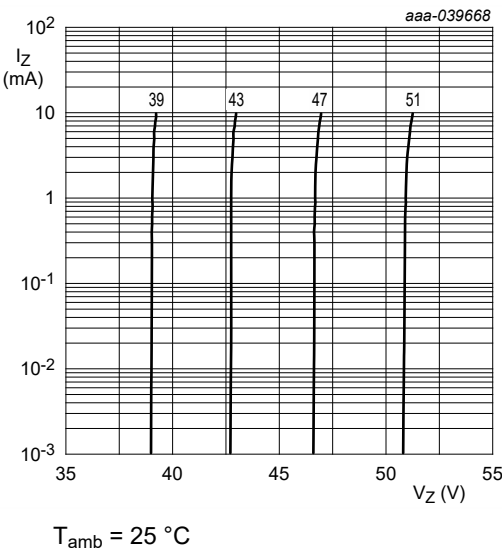
Fig. 8. Reverse current as a function of reverse voltage; typical values (BZX58550-B/C39-Q to BZX58550-B/C51-Q)
