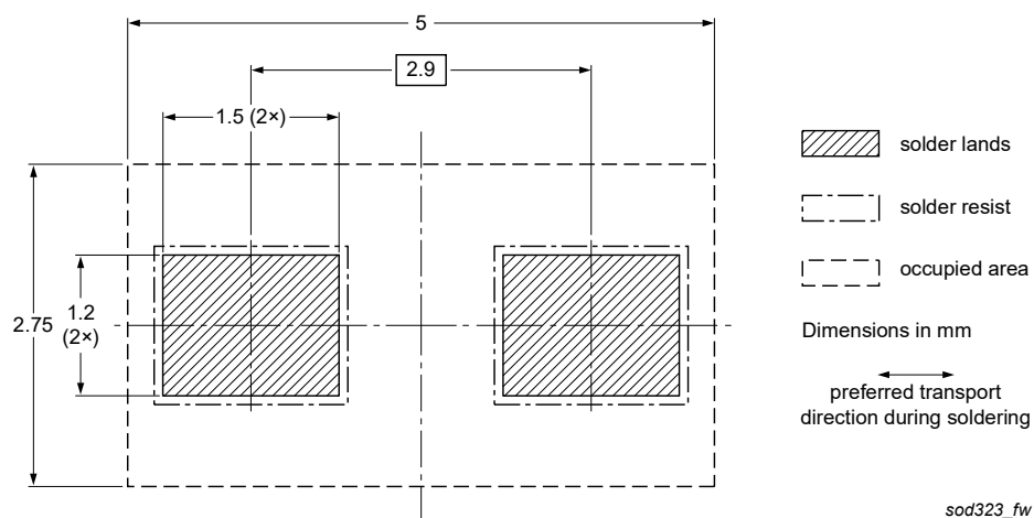
Fig. 11. Wave soldering footprint for SOD323 (SC-76)
