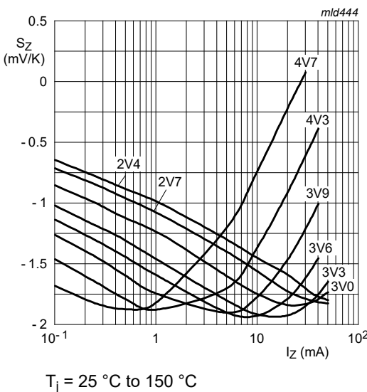
Fig. 6. Temperature coefficient as a function of working current; typical values (BZT52-B/C2V4-Q to B/C4V7-Q)
