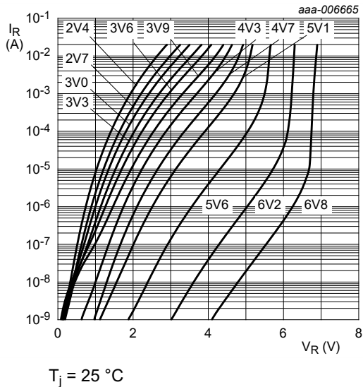
Fig. 8. Reverse current as a function of reverse voltage; typical values (BZT52-B/C2V4-Q to -B/C6V8-Q)
