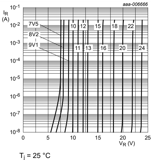
Fig. 9. Reverse current as a function of reverse voltage; typical values (BZT52-B/C7V5-Q to B/C24-Q)
