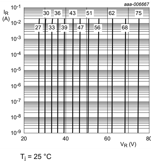
Fig. 10. Reverse current as a function of reverse voltage; typical values (BZT52-B/C27-Q to -B/C75-Q)
