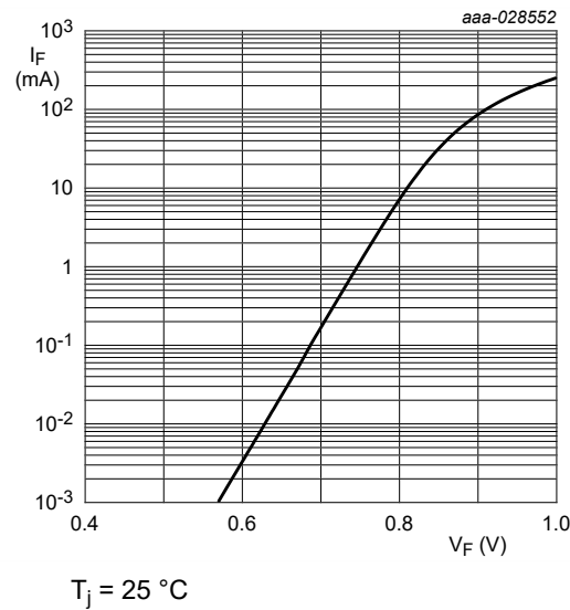
Fig. 4. Forward current as a function of forward voltage; typical values (BZT52-B/C7V5-Q)
