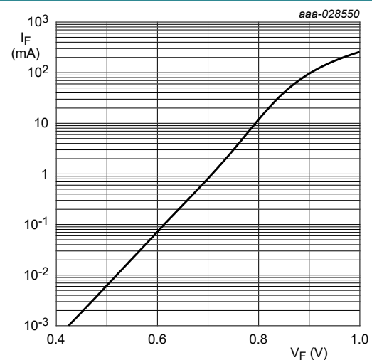
Fig. 2. Forward current as a function of forward voltage; typical values (BZT52-B/C2V4-Q)
