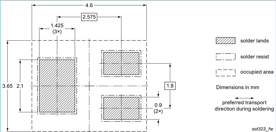
Fig. 6. Wave soldering footprint for SC-70 (SOT323)
