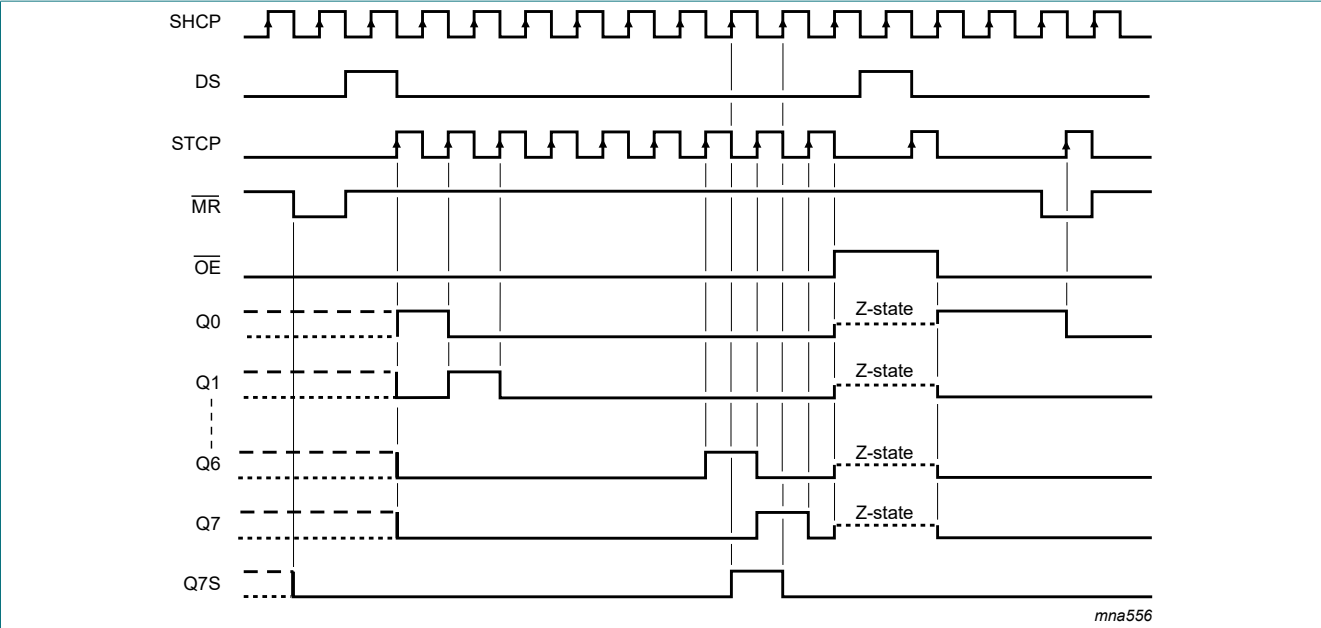
Fig. 7. Timing diagram
